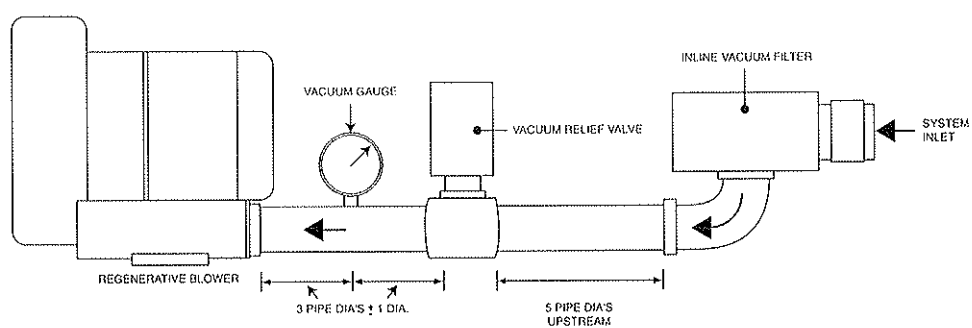
Typical Vacuum System
